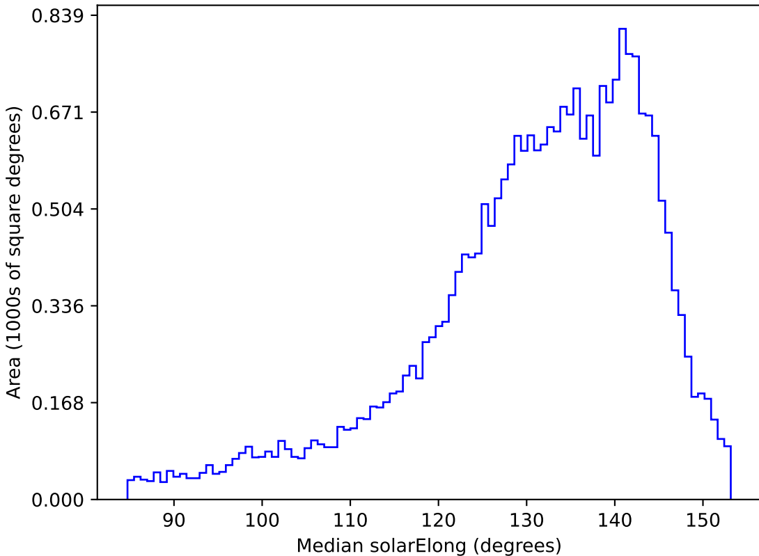
too_5_1v3.4_10yrs All sky r band: Median solarElong
