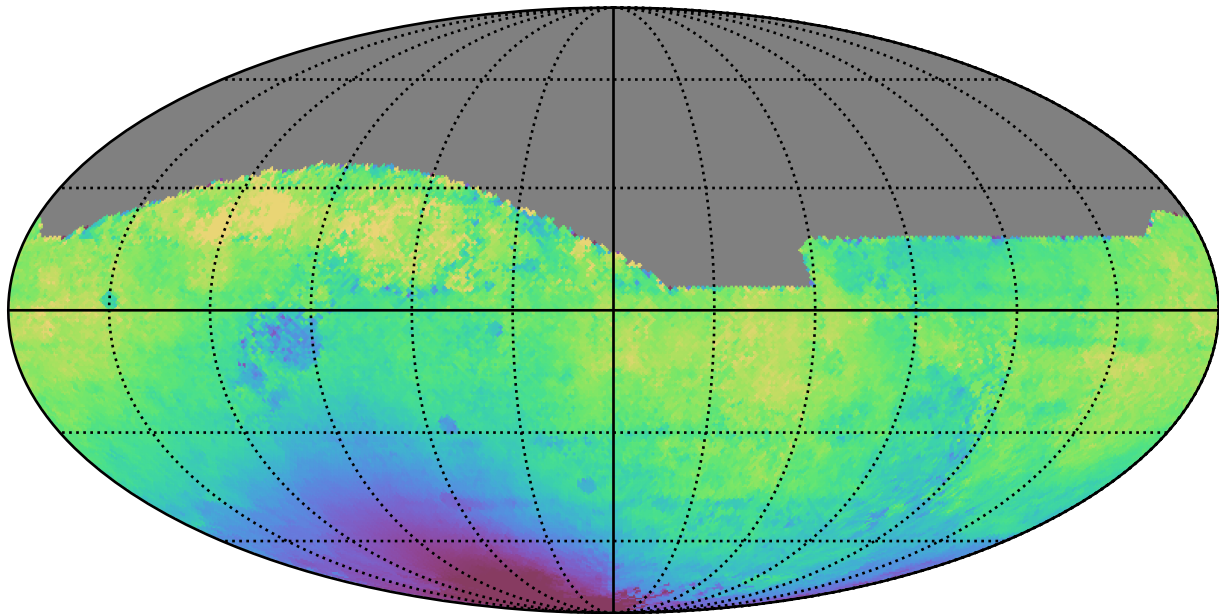
too_5_1v3.4_10yrs All sky i band: Median solarElong
