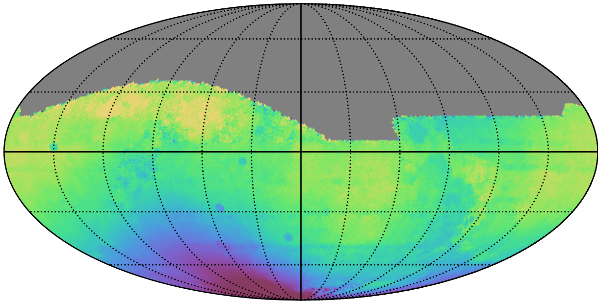
too_5_1v3.4_10yrs All sky all bands: Median solarElong
