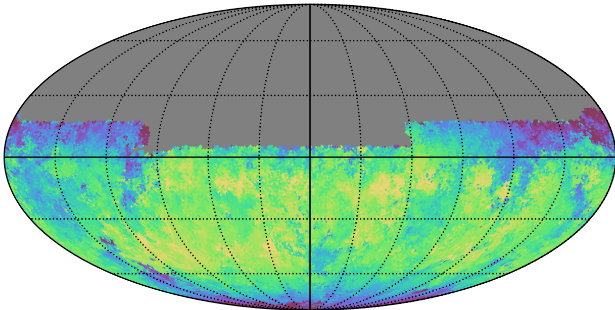
too_5_1v3.4_10yrs Yr 1 y band: Median skyBrightness
