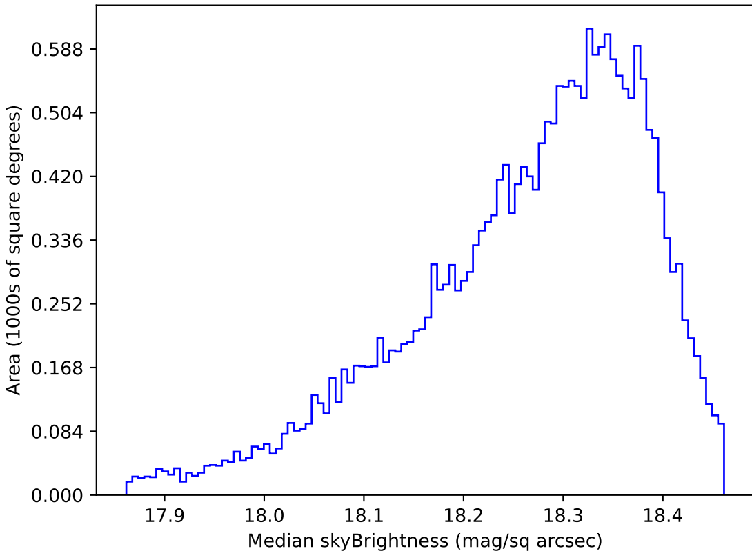
too_5_1v3.4_10yrs Yr 1 y band: Median skyBrightness
