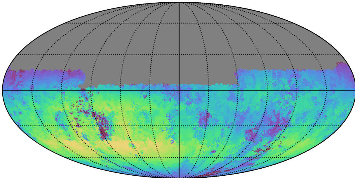
too_5_1v3.4_10yrs Yr 1 u band: Median skyBrightness
