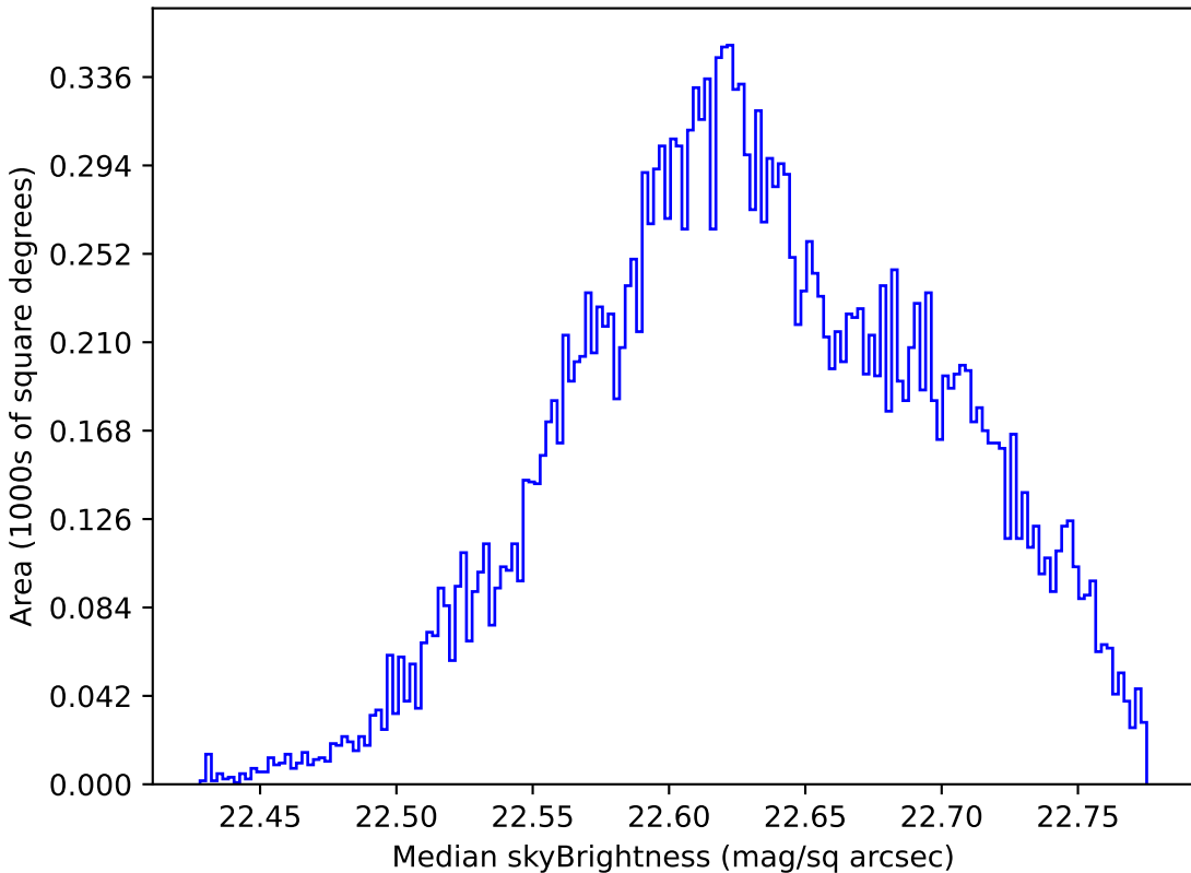
too_5_1v3.4_10yrs Yr 1 u band: Median skyBrightness
