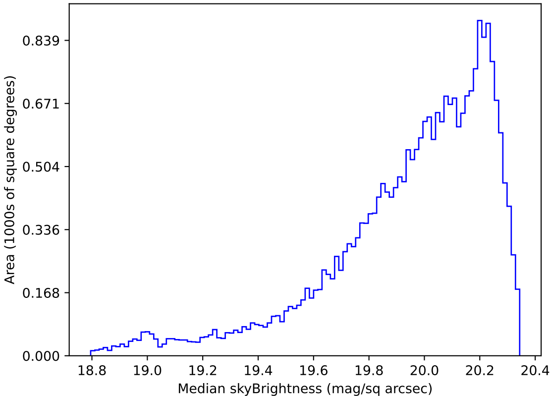
too_5_1v3.4_10yrs Yr 1 i band: Median skyBrightness
