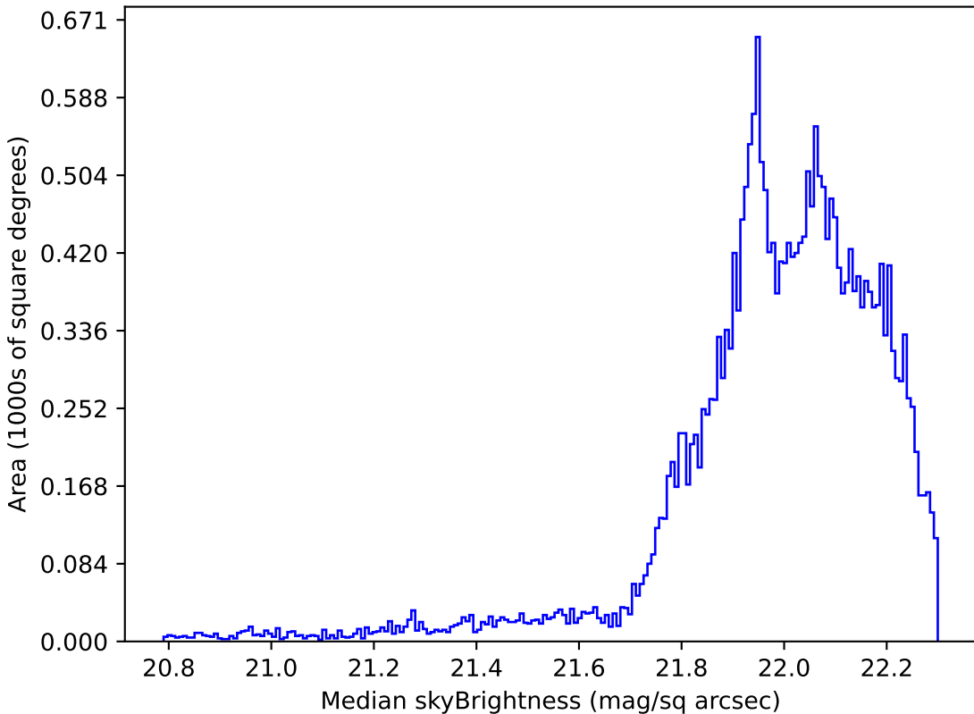
too_5_1v3.4_10yrs Yr 1 g band: Median skyBrightness
