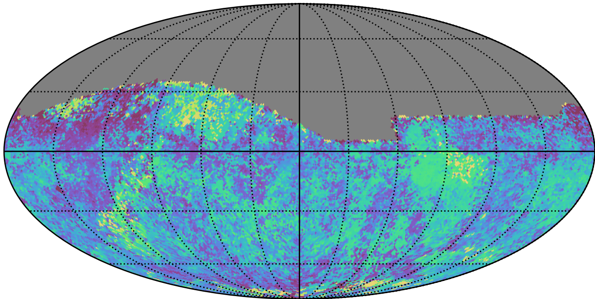
too_5_1v3.4_10yrs Yr 1 all bands: Median skyBrightness
