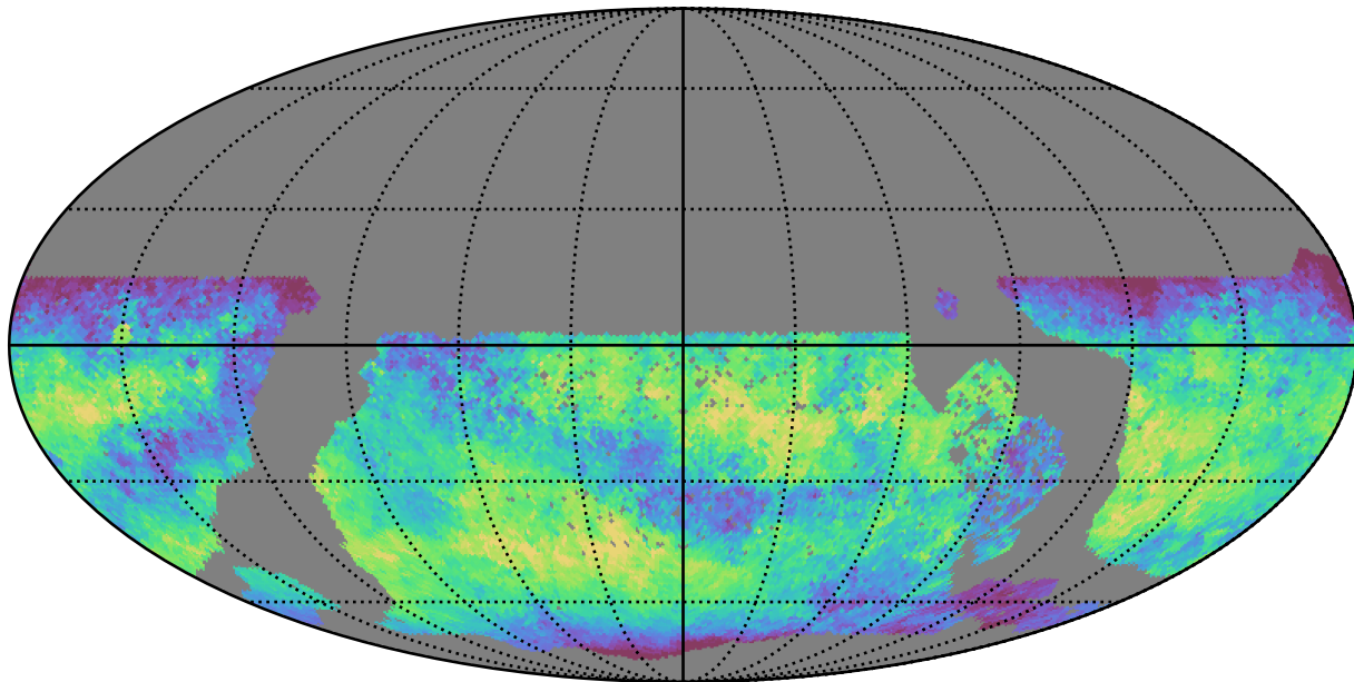
too_5_1v3.4_10yrs WFD z band: Median skyBrightness
