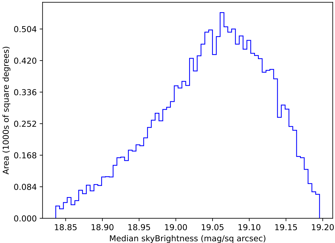
too_5_1v3.4_10yrs WFD z band: Median skyBrightness
