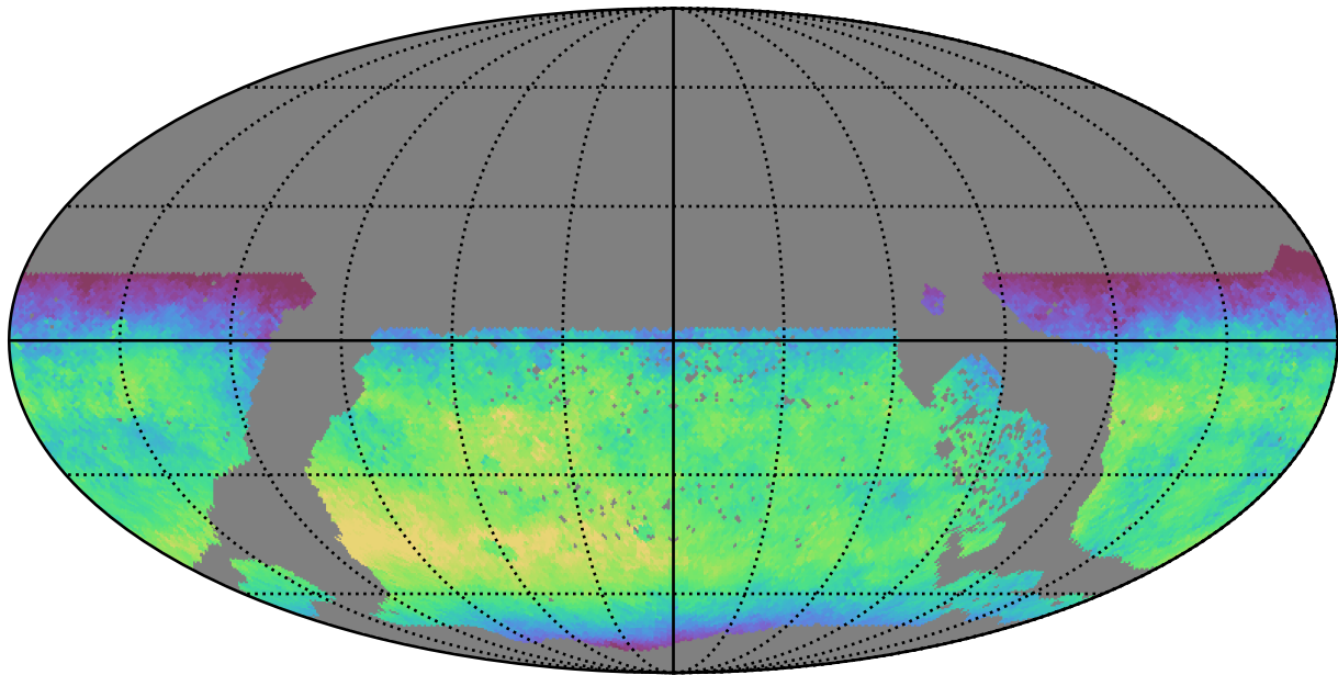
too_5_1v3.4_10yrs WFD y band: Median skyBrightness
