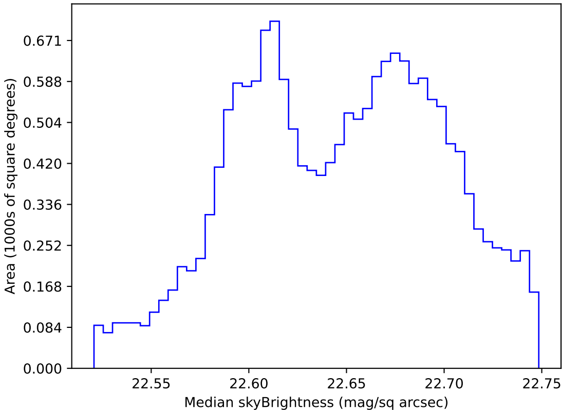
too_5_1v3.4_10yrs WFD u band: Median skyBrightness
