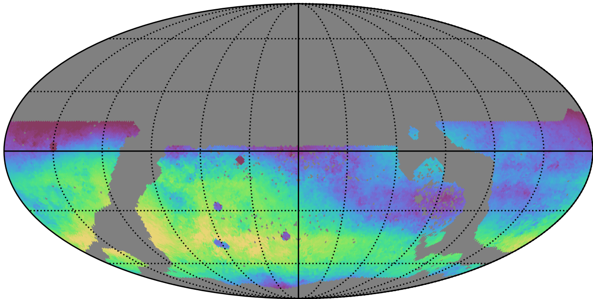
too_5_1v3.4_10yrs WFD r band: Median skyBrightness
