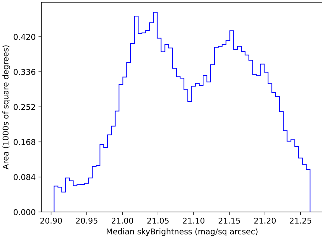
too_5_1v3.4_10yrs WFD r band: Median skyBrightness
