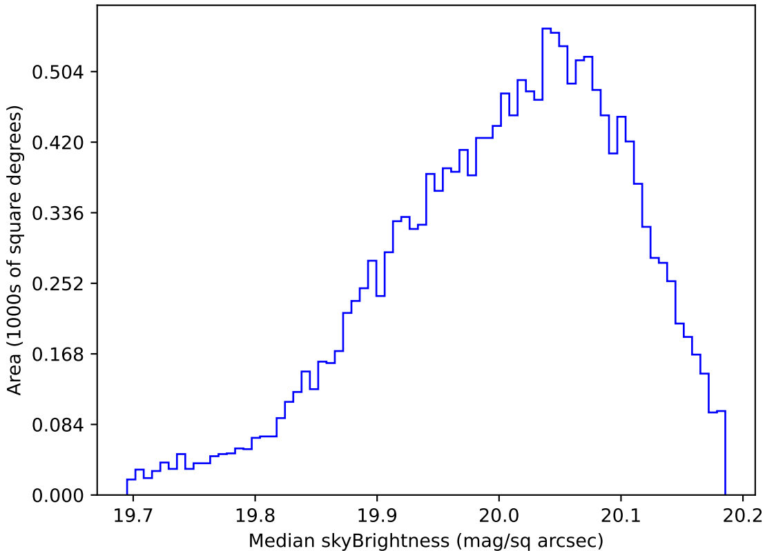
too_5_1v3.4_10yrs WFD i band: Median skyBrightness
