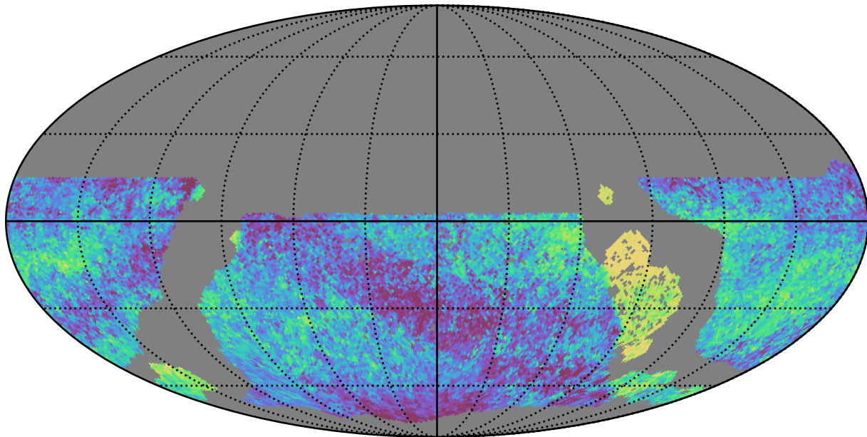
too_5_1v3.4_10yrs WFD all bands: Median skyBrightness
