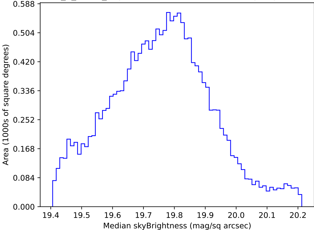
too_5_1v3.4_10yrs WFD all bands: Median skyBrightness
