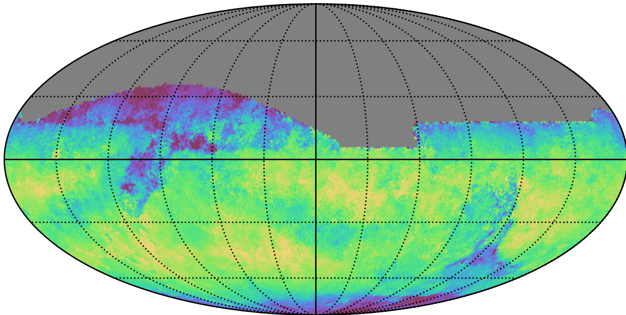
too_5_1v3.4_10yrs All sky z band: Median skyBrightness
