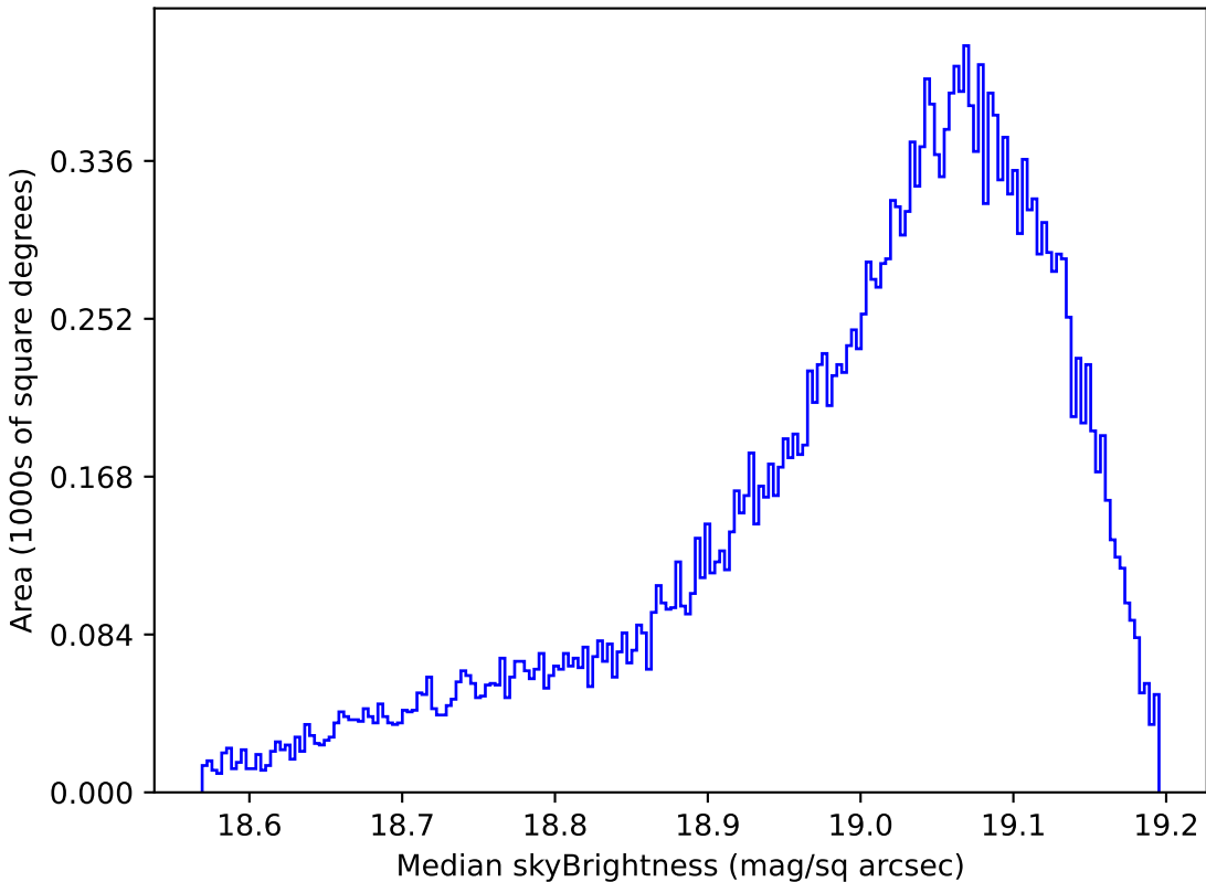
too_5_1v3.4_10yrs All sky z band: Median skyBrightness
