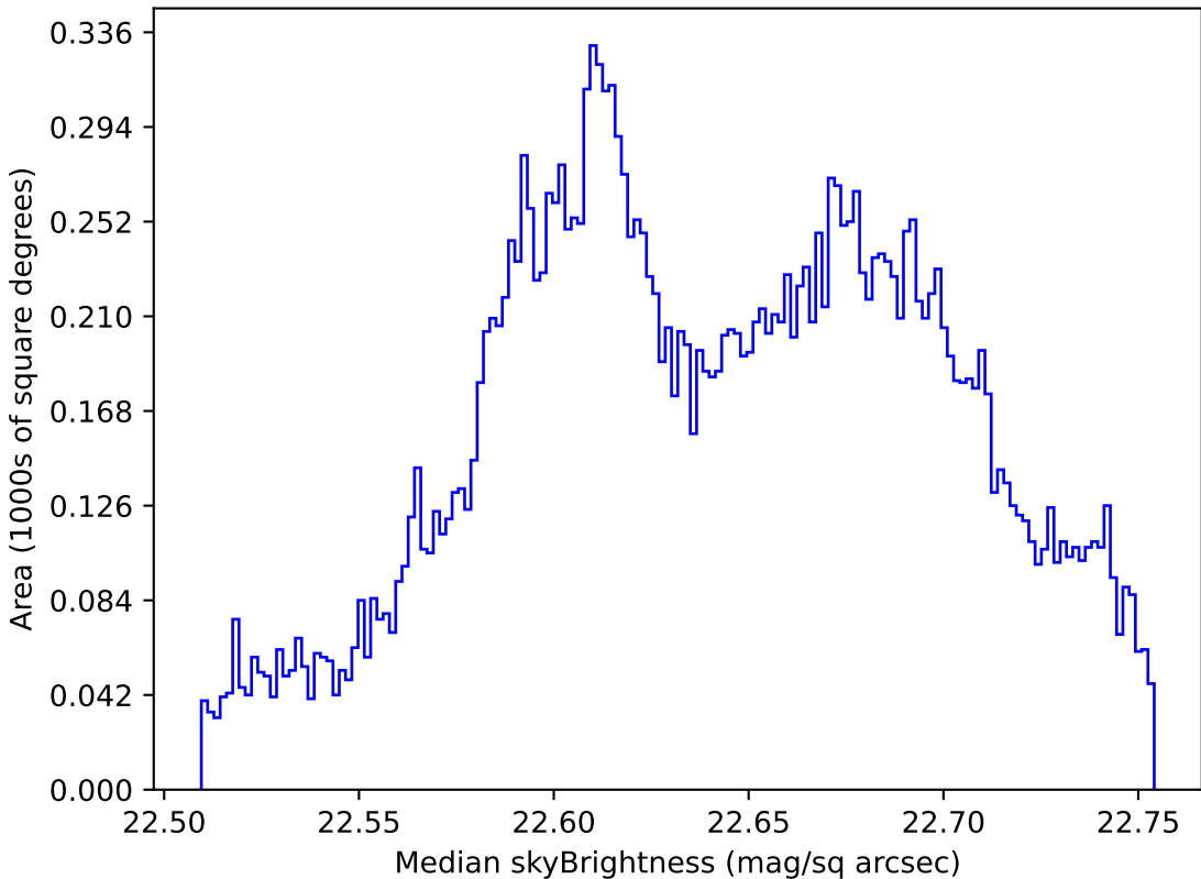
too_5_1v3.4_10yrs All sky u band: Median skyBrightness
