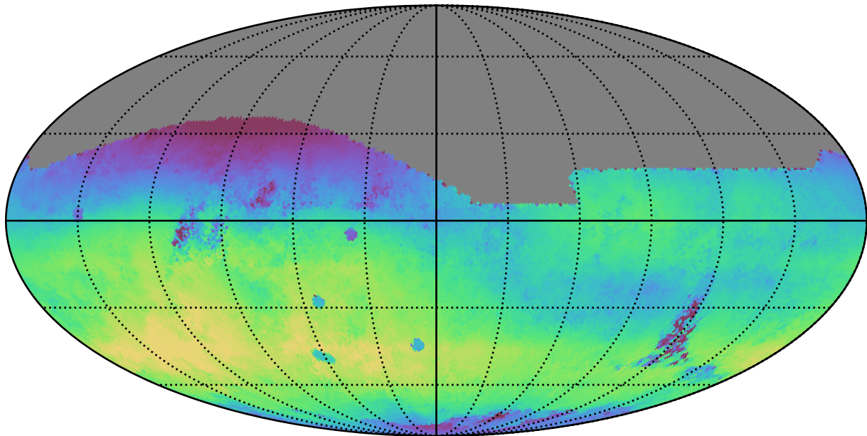
too_5_1v3.4_10yrs All sky r band: Median skyBrightness
