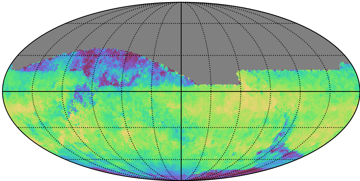
too_5_1v3.4_10yrs All sky i band: Median skyBrightness
