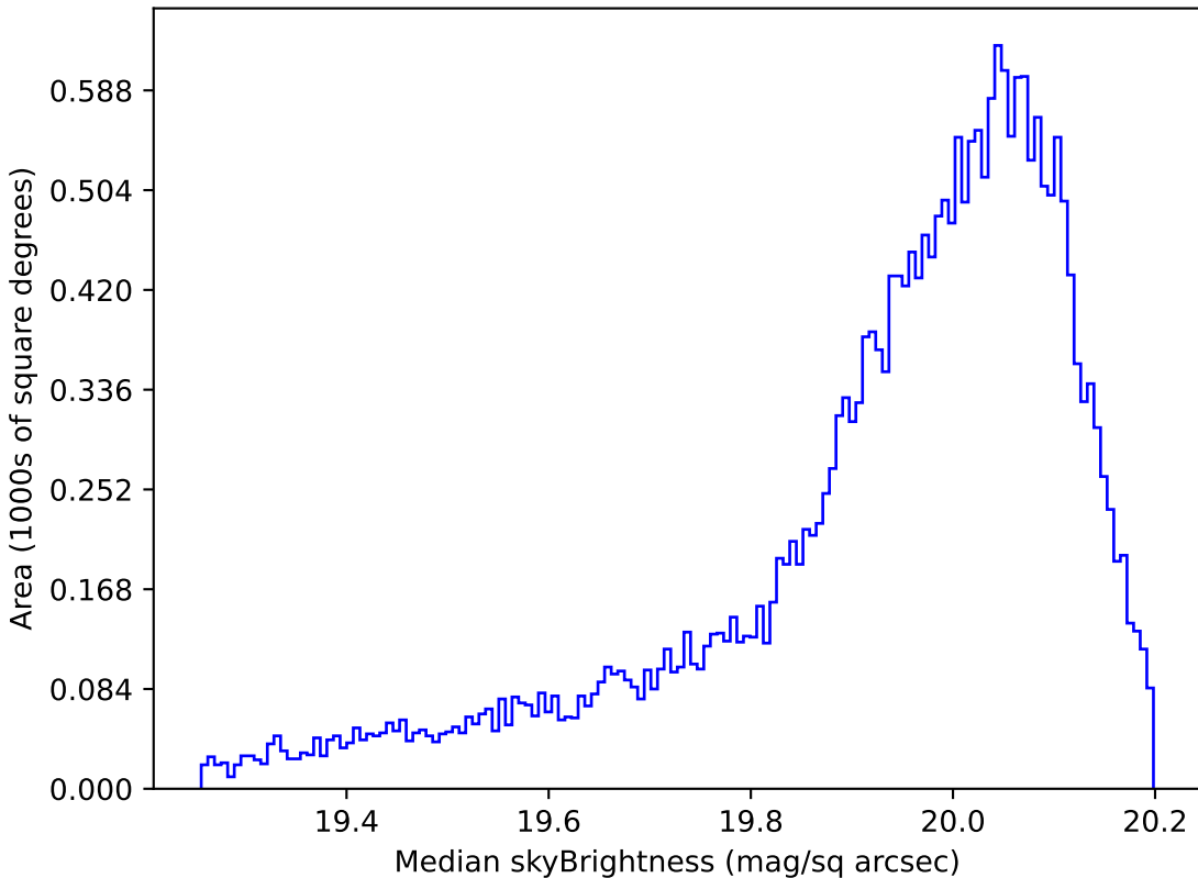
too_5_1v3.4_10yrs All sky i band: Median skyBrightness
