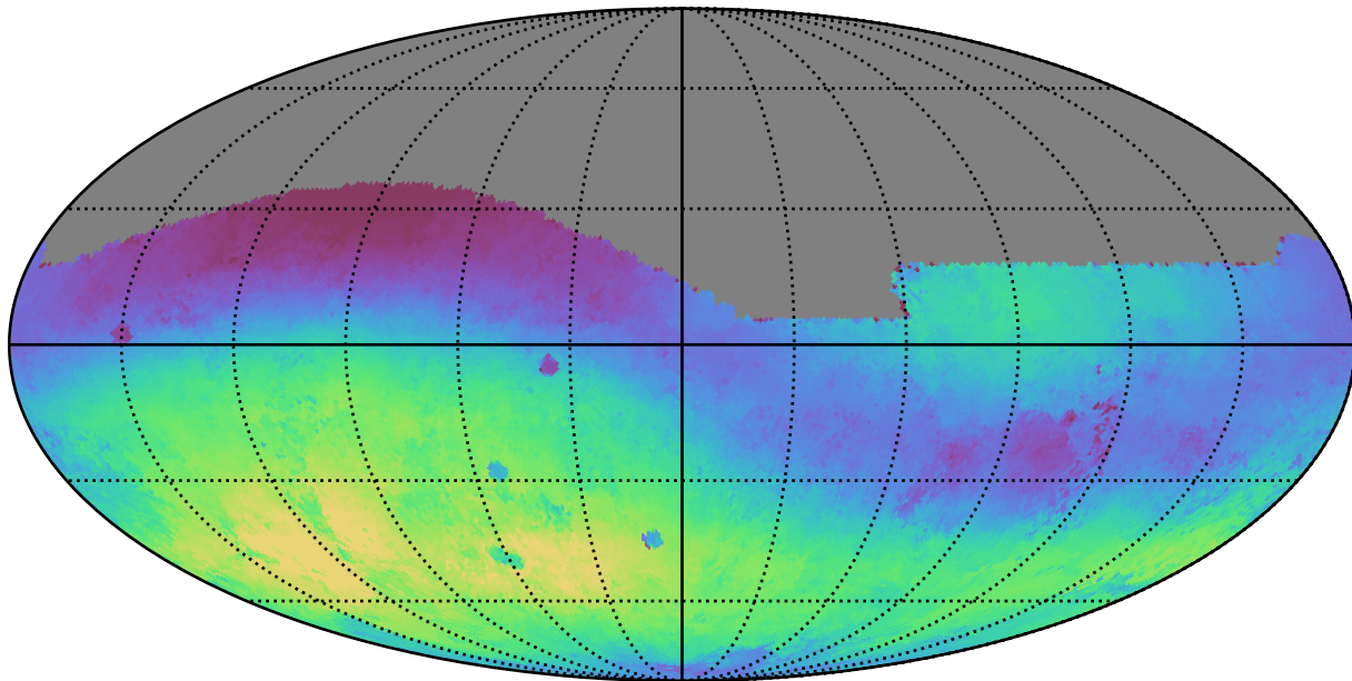
too_5_1v3.4_10yrs All sky g band: Median skyBrightness
