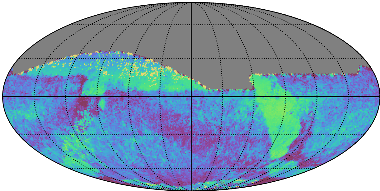
too_5_1v3.4_10yrs All sky all bands: Median skyBrightness
