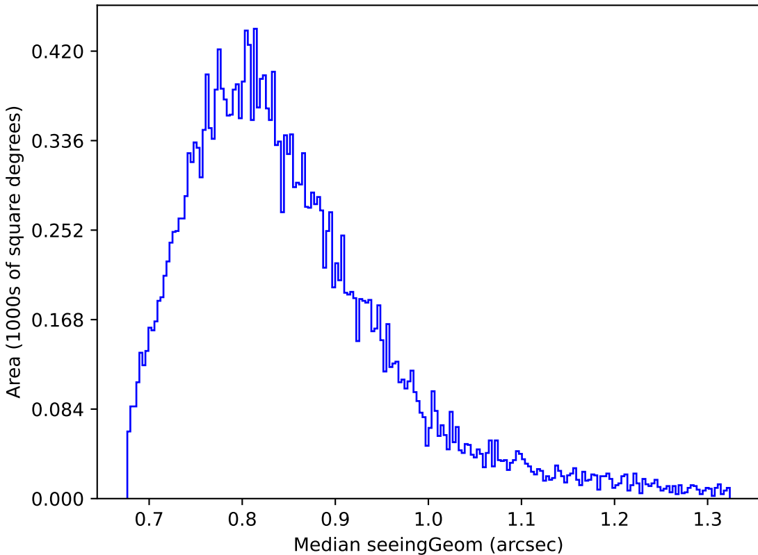
too_5_1v3.4_10yrs Yr 1 z band: Median seeingGeom
