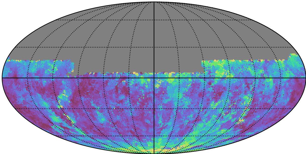
too_5_1v3.4_10yrs Yr 1 y band: Median seeingGeom
