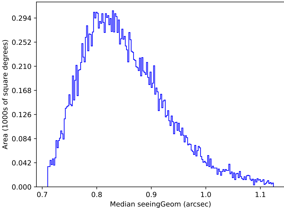
too_5_1v3.4_10yrs Yr 1 y band: Median seeingGeom
