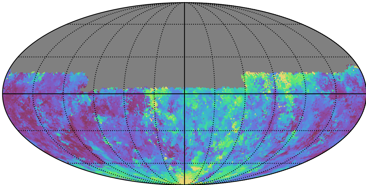
too_5_1v3.4_10yrs Yr 1 u band: Median seeingGeom
