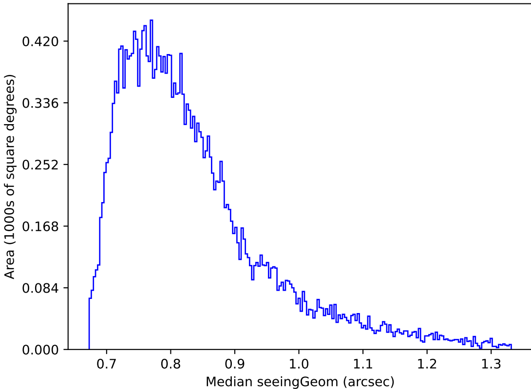
too_5_1v3.4_10yrs Yr 1 i band: Median seeingGeom
