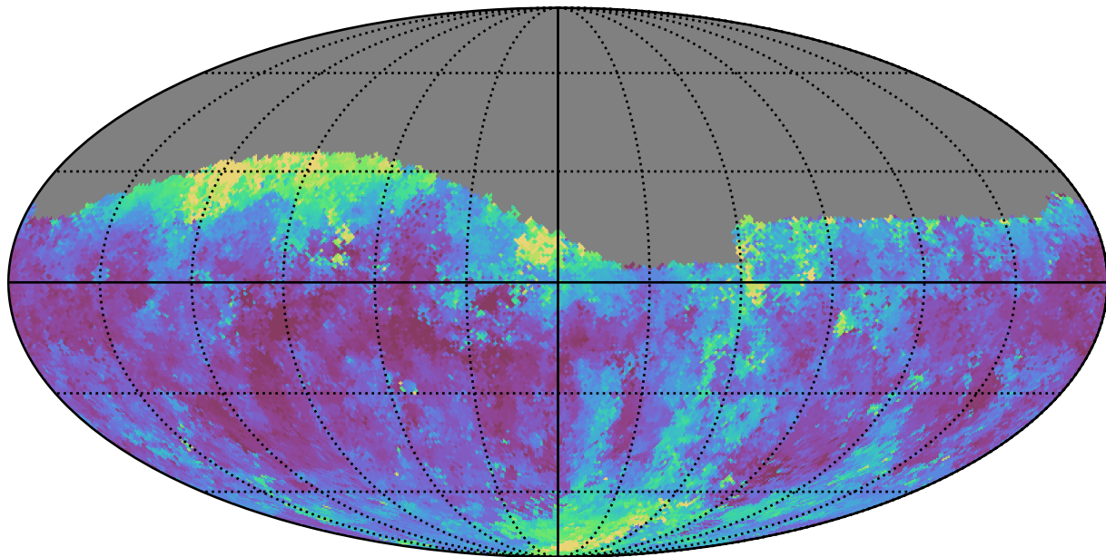
too_5_1v3.4_10yrs Yr 1 g band: Median seeingGeom
