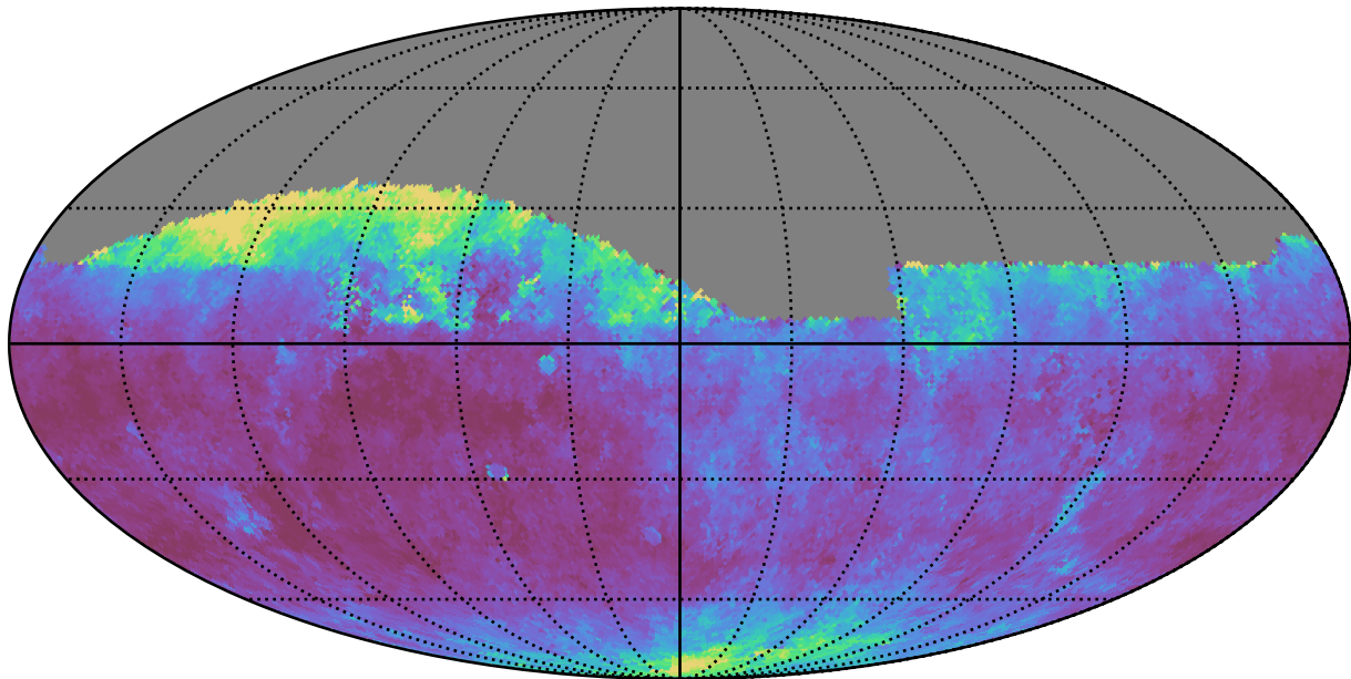
too_5_1v3.4_10yrs Yr 1 all bands: Median seeingGeom
