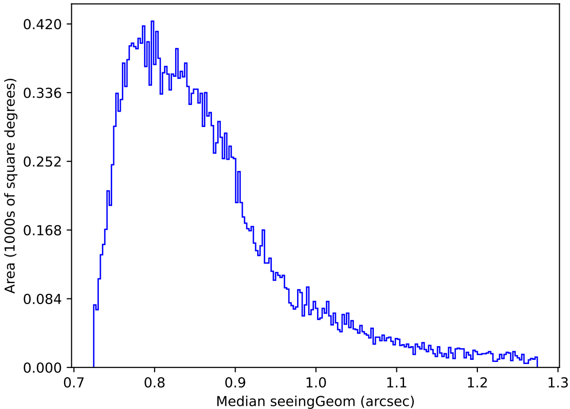
too_5_1v3.4_10yrs Yr 1 all bands: Median seeingGeom
