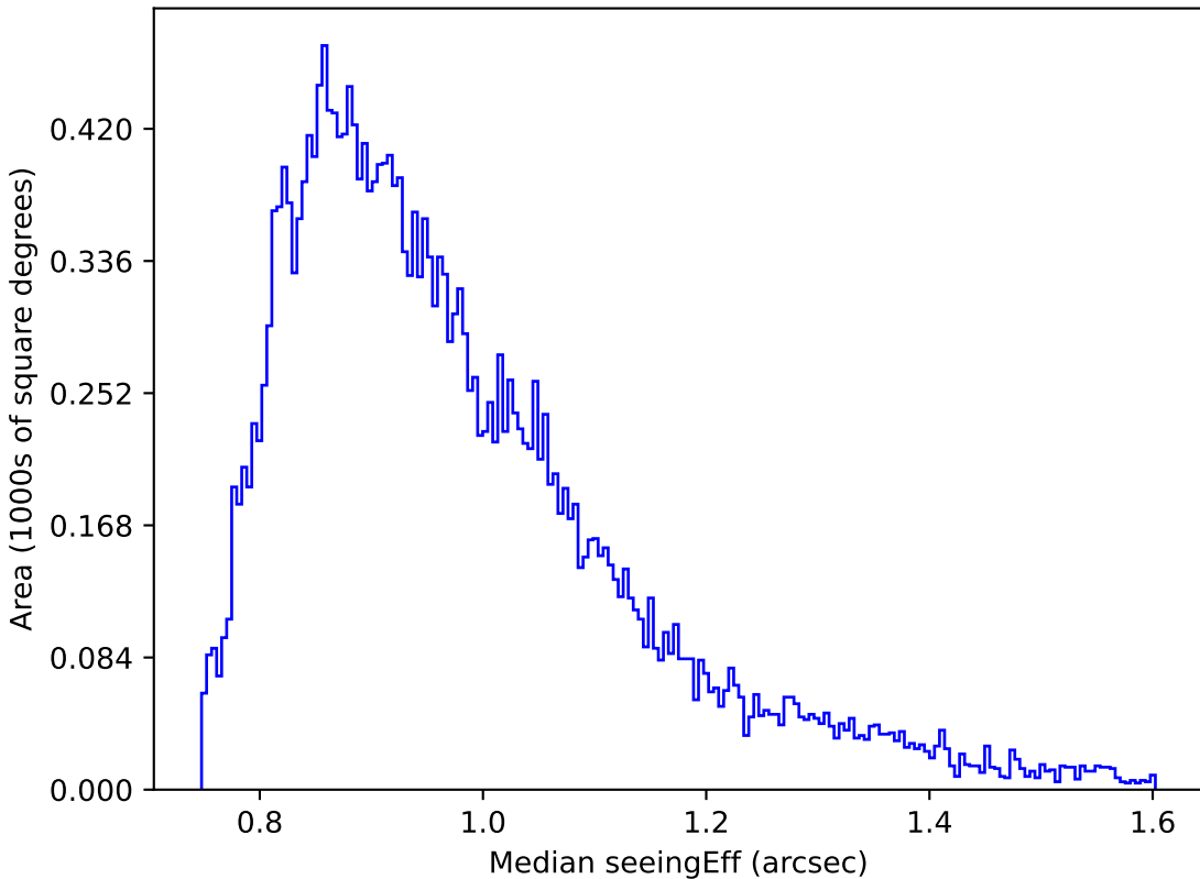
too_5_1v3.4_10yrs Yr 1 r band: Median seeingEff
