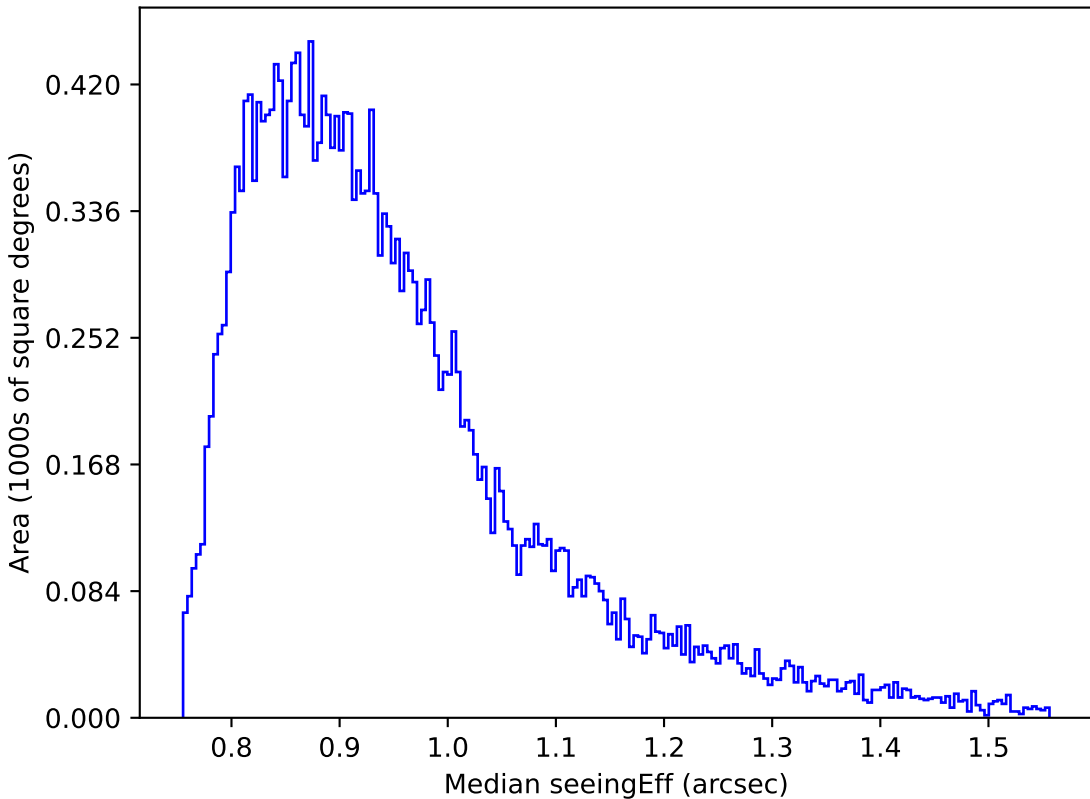
too_5_1v3.4_10yrs Yr 1 i band: Median seeingEff
