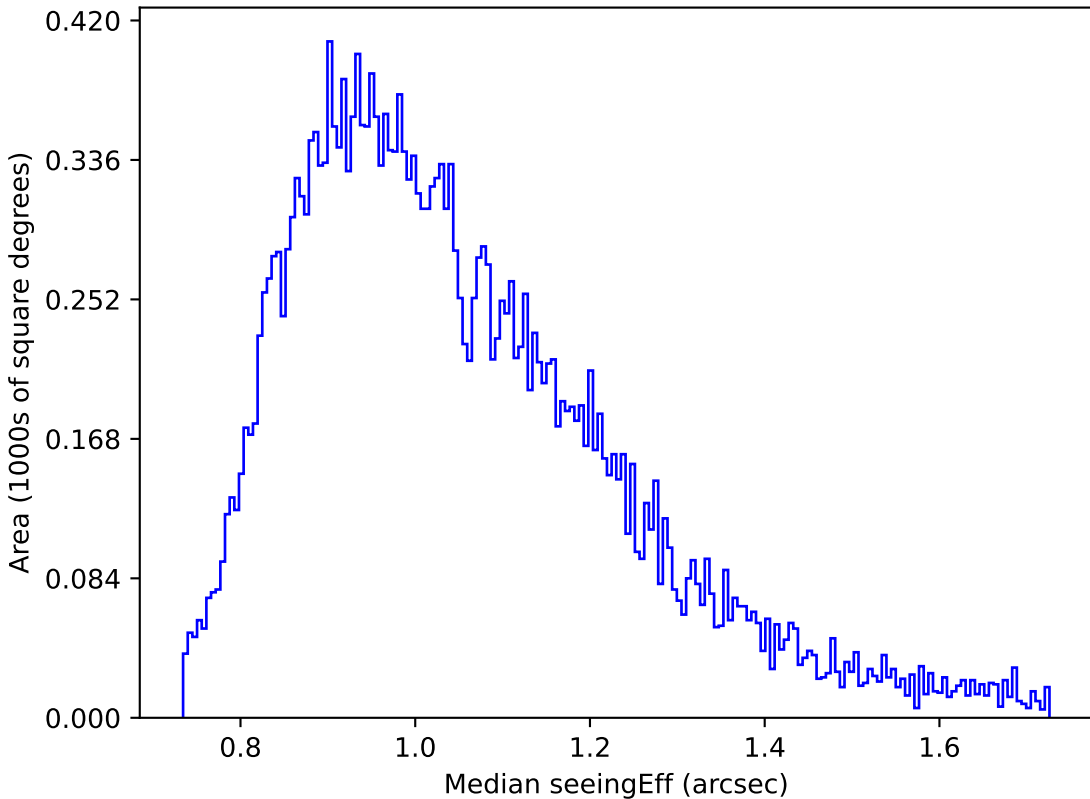
too_5_1v3.4_10yrs Yr 1 g band: Median seeingEff
