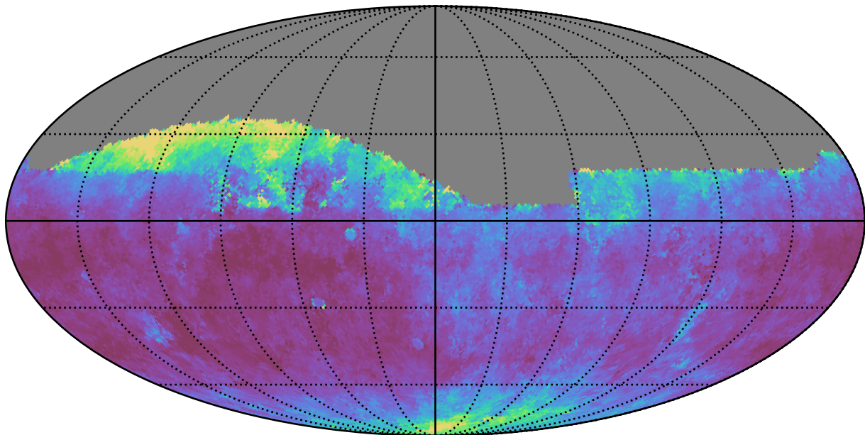
too_5_1v3.4_10yrs Yr 1 all bands: Median seeingEff
