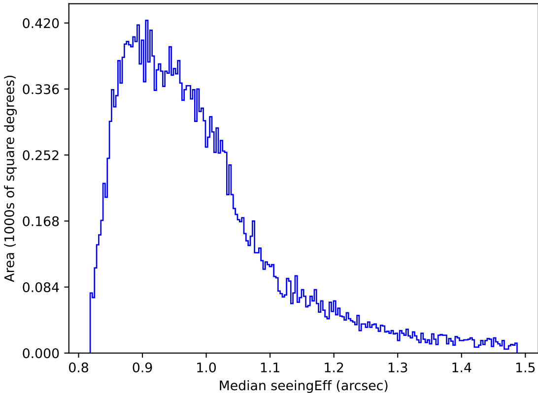
too_5_1v3.4_10yrs Yr 1 all bands: Median seeingEff
