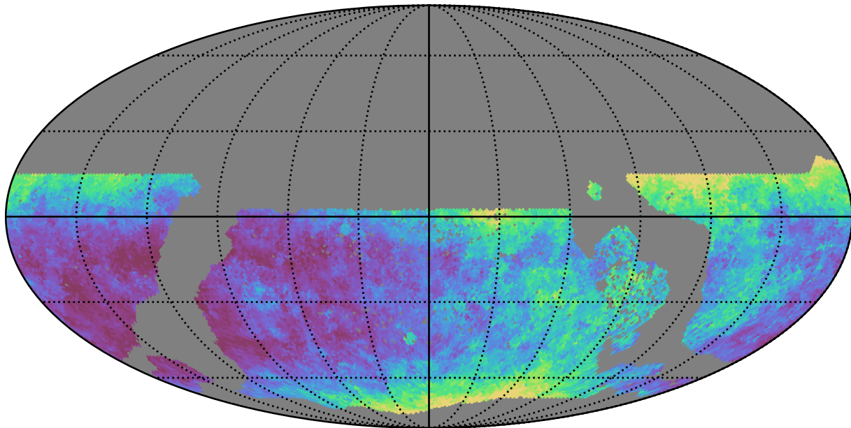
too_5_1v3.4_10yrs WFD y band: Median seeingEff
