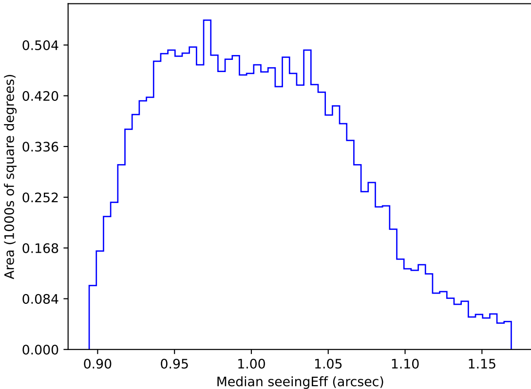
too_5_1v3.4_10yrs WFD y band: Median seeingEff
