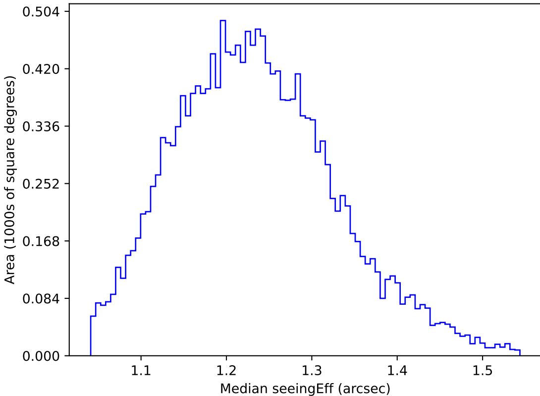
too_5_1v3.4_10yrs WFD u band: Median seeingEff
