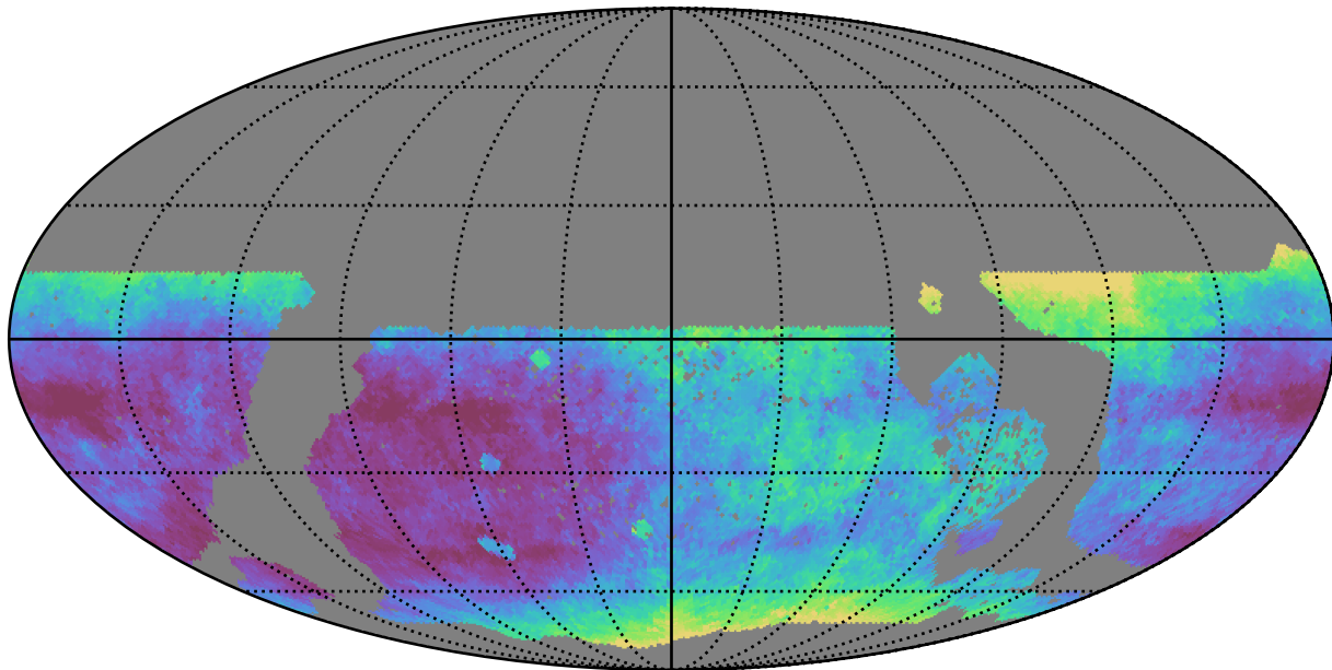
too_5_1v3.4_10yrs WFD r band: Median seeingEff
