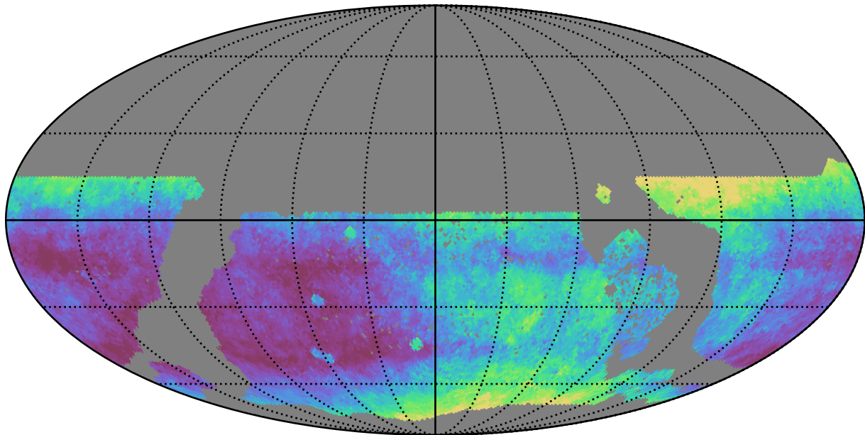
too_5_1v3.4_10yrs WFD i band: Median seeingEff
