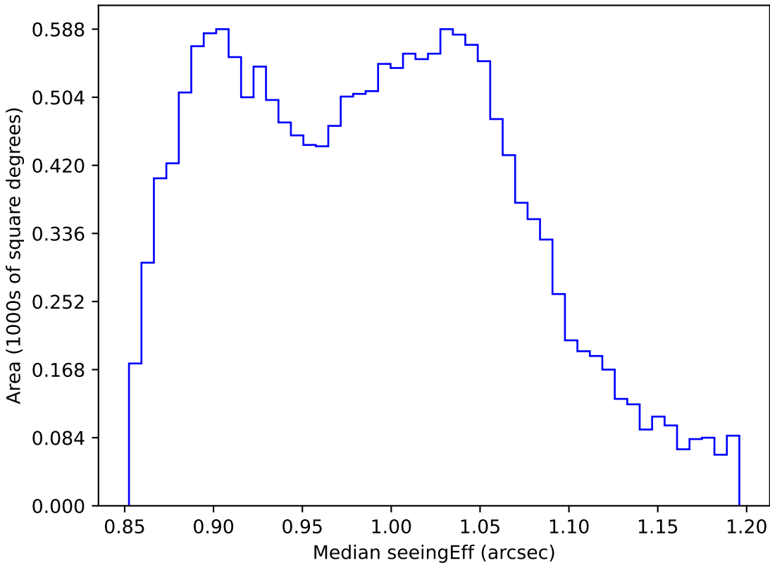
too_5_1v3.4_10yrs WFD i band: Median seeingEff
