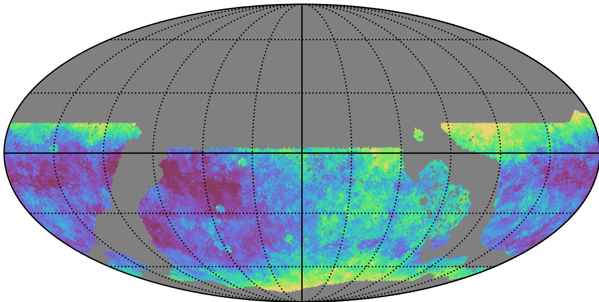
too_5_1v3.4_10yrs WFD g band: Median seeingEff
