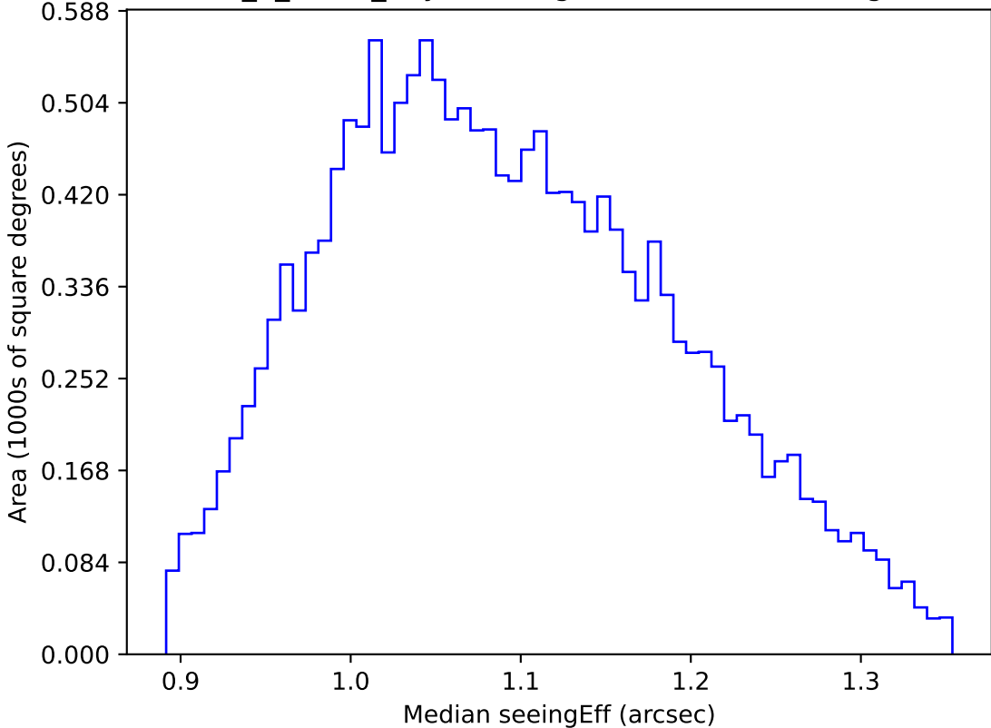
too_5_1v3.4_10yrs WFD g band: Median seeingEff
