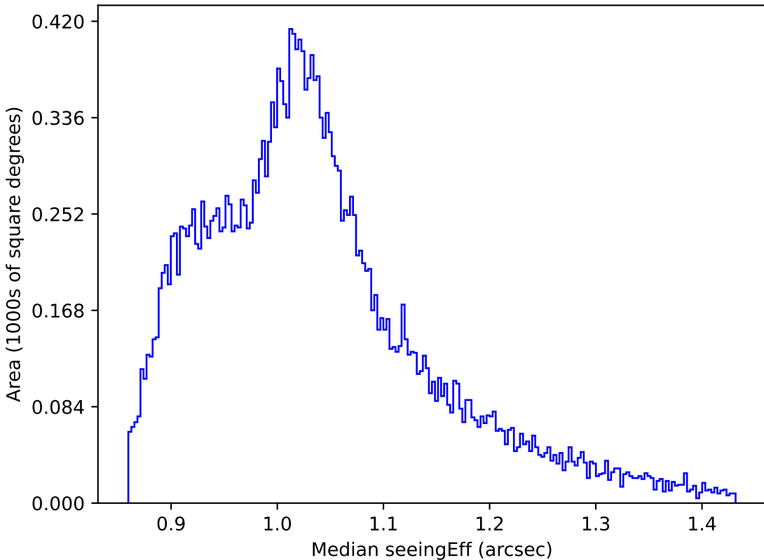
too_5_1v3.4_10yrs All sky z band: Median seeingEff
