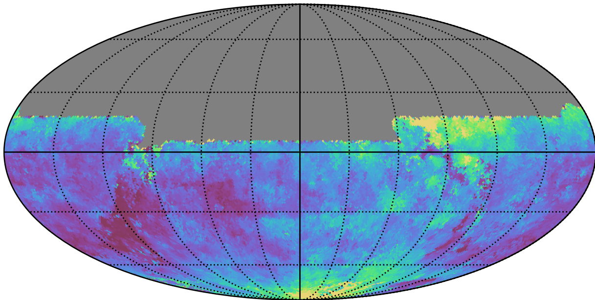
too_5_1v3.4_10yrs All sky u band: Median seeingEff
